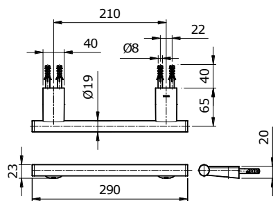
TX702ARR "REI R" Hand Towel Bar
