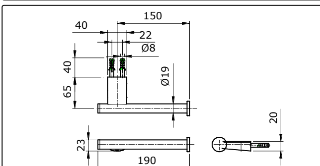
TX703ARR "REI R" Paper Holder
