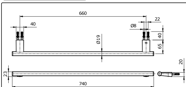
TX701ARR "REI R" Towel Bar
