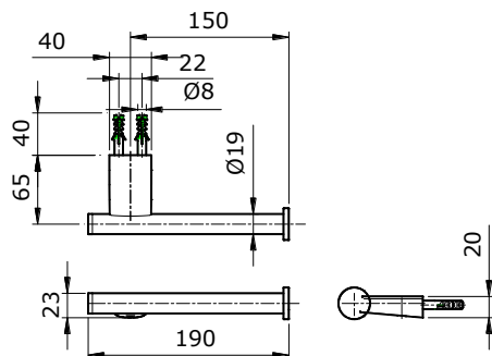
TX703ARR "REI R" Paper Holder
