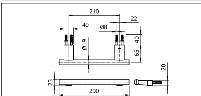
TX702ARR "REI R" Hand Towel Bar
